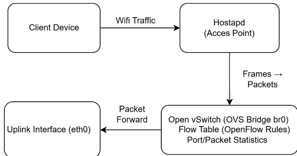
Gambar 2. 3 Diagram Blok Subsistem 1
