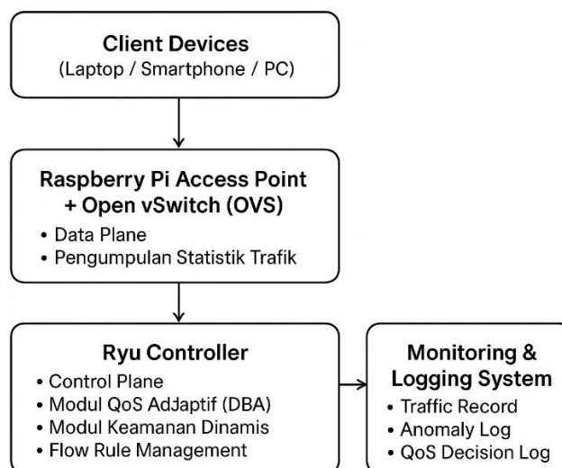
Gambar 2. 1 Blok Diagram System
